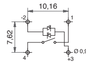
Bicolor - 2 LEDs
