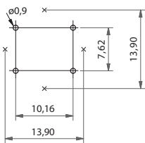
5E+1YS/1YAS - TH
