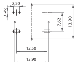
5E+1YS/1YAS - SMD
