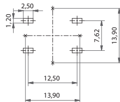
3E+1Y/1YA - SMD
