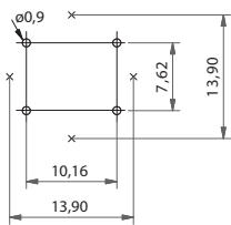
3E+1Y/1YA - TH
